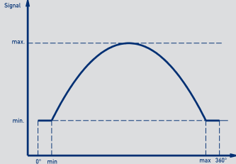
On request: Parabolic output characteristic
